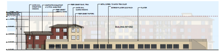
ALLEY (WEST) ELEVATION
