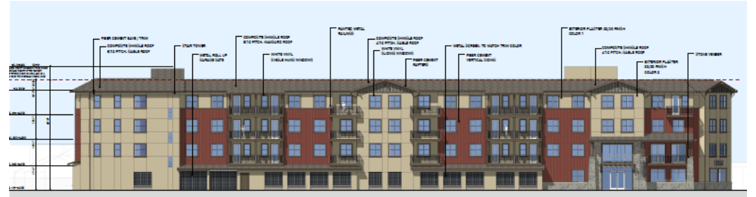
SAN ANTONIO DRIVE (EAST) ELEVATION
