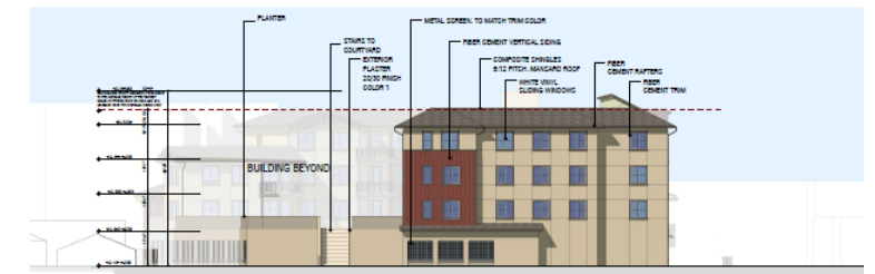
PARKING LOT (SOUTH) ELEVATION
